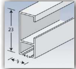
HANGING RAIL
